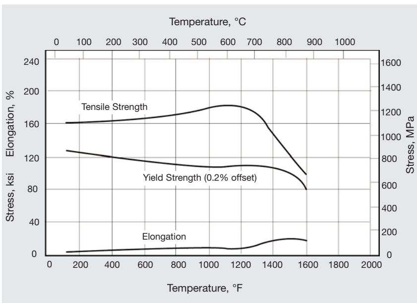
Figure 1 , Typical mechanical properties of precipitation-hardened LION alloy 720
