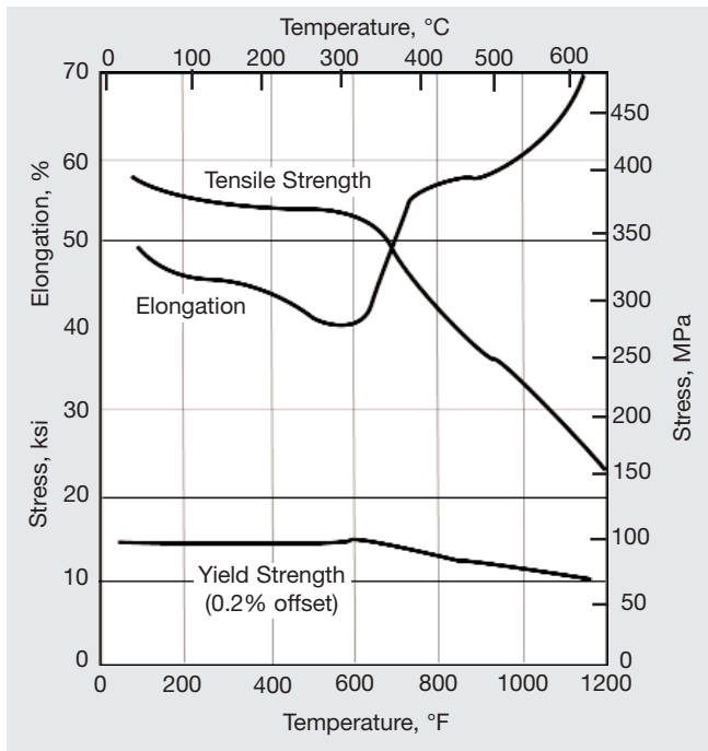
Figure 12 - High-temperature tensile properties of annealed Nickel 201.
